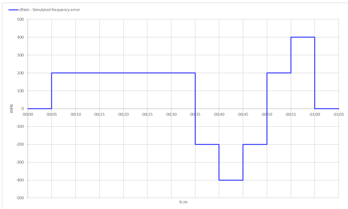
Figure 10. Simulated frequency profile for the dynamic characterization of frequency control deployment
