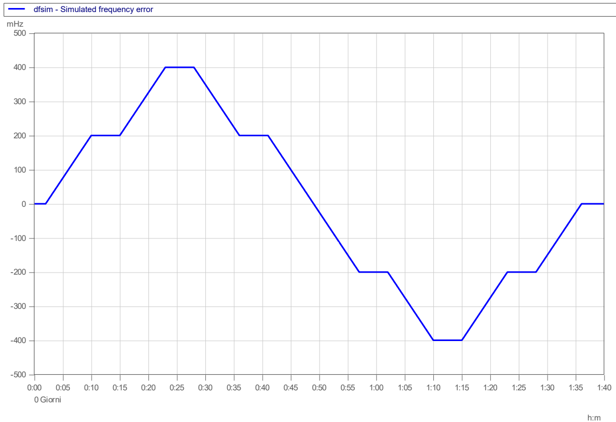
Figure 9. Simulated frequency profile for the static characterization of the frequency control
