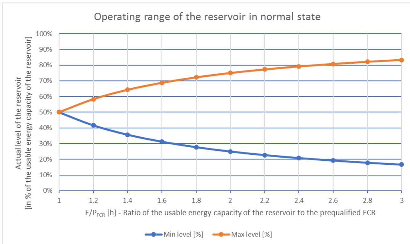
Figure 7. Management of the energy reservoir of a FCR providing unit with LER
