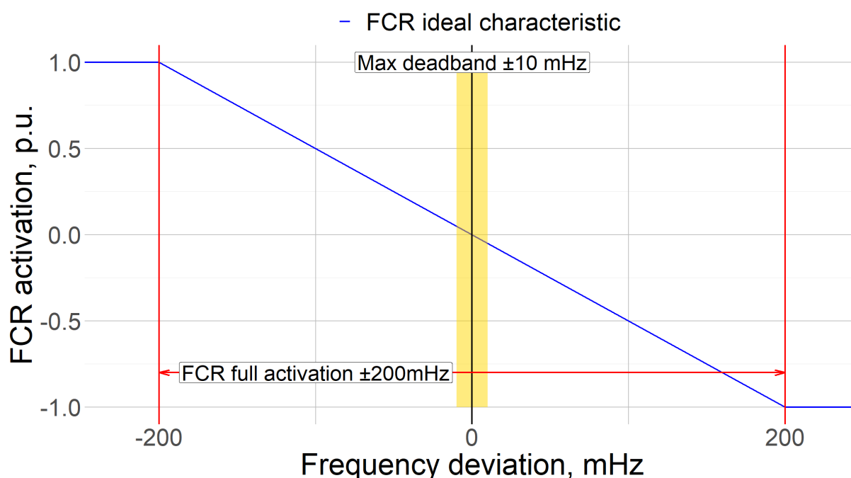
Figure 2. Static frequency deviation / FCR activation example curves
