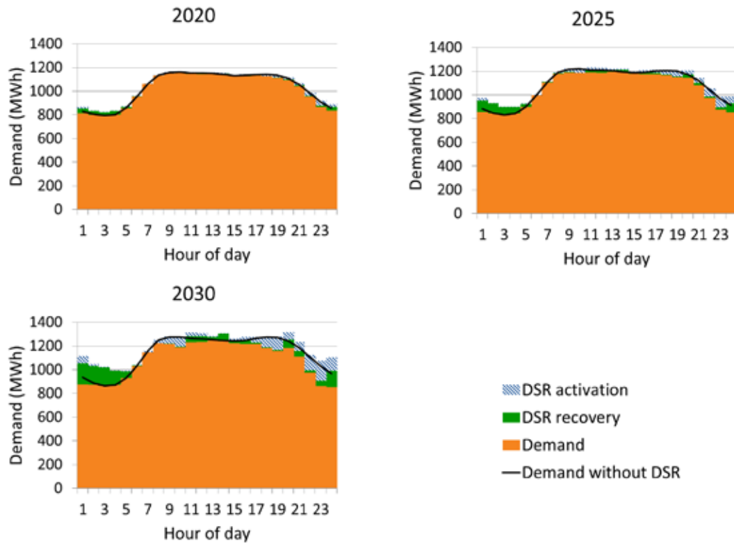
Figure 30 – Average daily use of DSR
