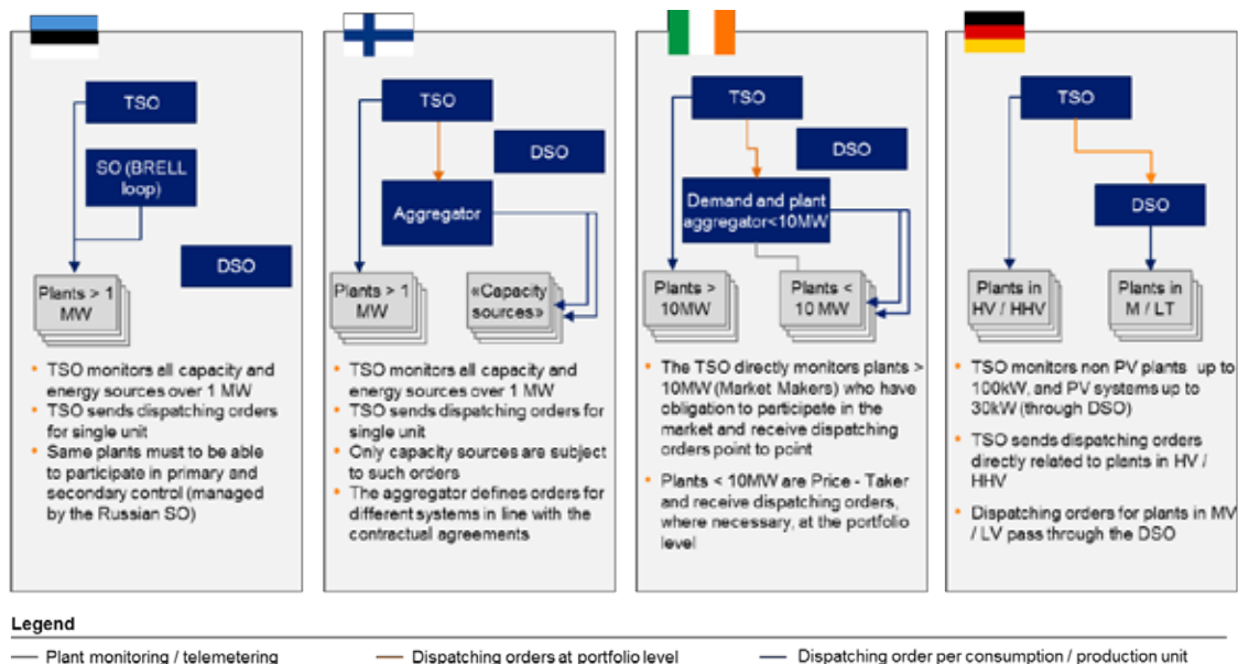
Figure 22 – TSO-DSO interaction in balancing activities in selected countries
