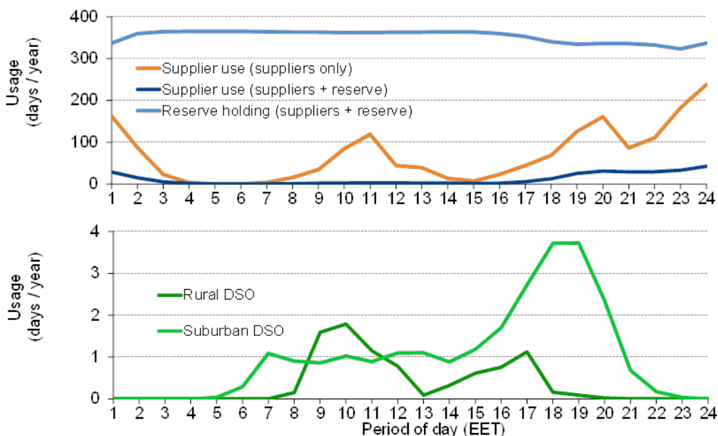
Figure 63 – DSR calling patterns (Estonia, 2030)
